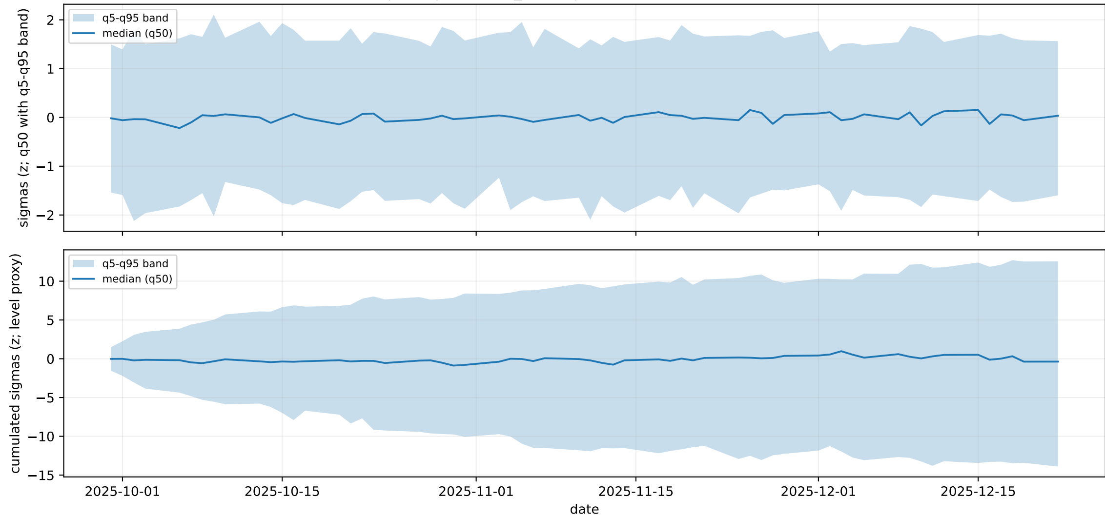
latest | USA | systemic_stress | block aggregate quantile bands
